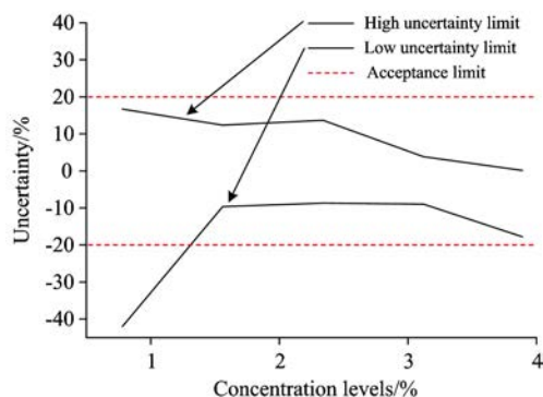
Fig. 2 Uncertainty profile
