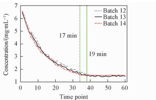
Fig. 6 HPLC validation for the end-point detection of the alcohol adding process
