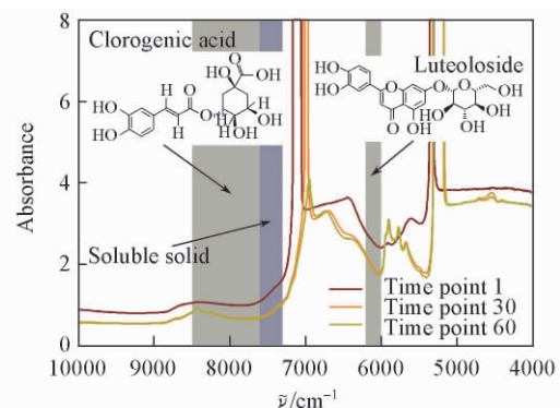
Fig. 2 Raw NIR spectra with the characteristic wave-band during the alcohol precipitation process
