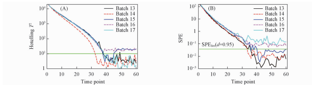
Fig. 5 End-point detection of the alcohol adding process for Batches 13 to 17
