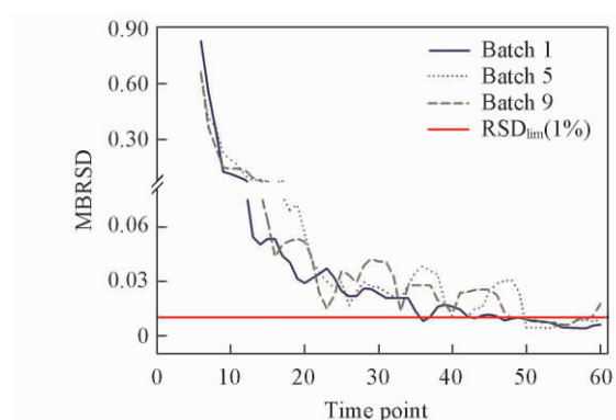
Fig. 3 Selection of end-points from the alcohol adding process under normal operating conditions by PCA-MBRSD
